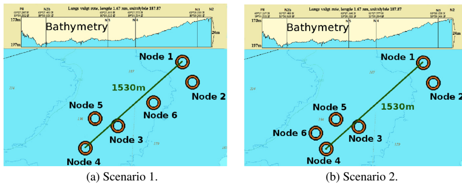
Fig. 4. Network topologies for pipeline and oil well monitoring.
