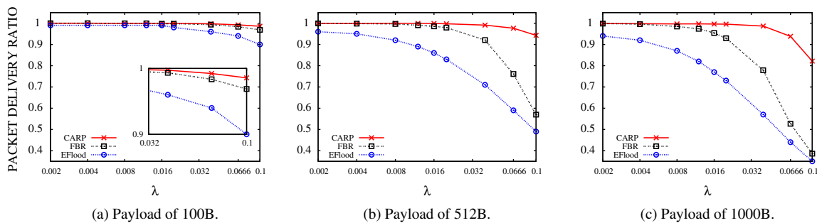
Fig. 1. Packet delivery ratio.
