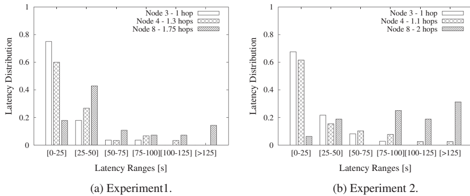
Fig. 6. CARP: end-to-end latency distribution for traffic sources.
