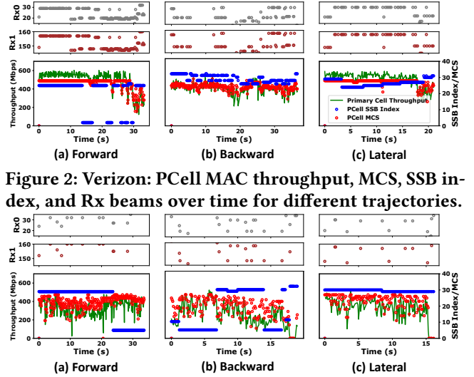
Figure 3: AT&T: PCell MAC throughput, MCS, SSB index, and Rx beams over time for different trajectories.
