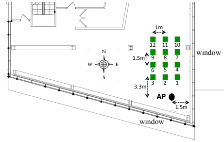
Figure 8: Experimental floorplan. Square boxes represent client positions.
