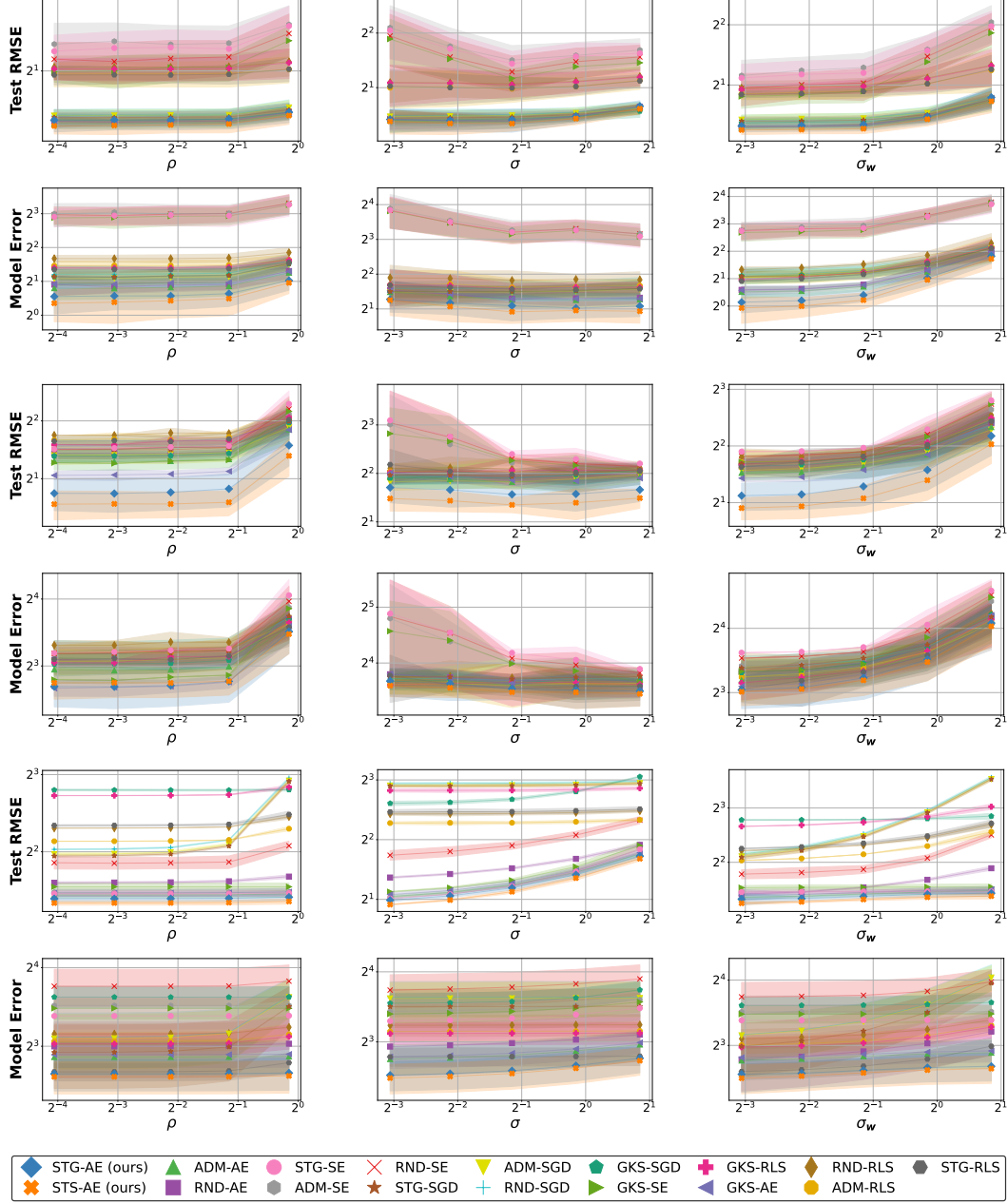
Figure 9: Test RMSE (Eq. (145)) and model error (Eqs. (147)–(148)) comparisons with respect to different values of \rho , \sigma , and \sigma_w on the synthetic dataset, for the CNN (rows 1–2), MLP (rows 3–4), and linear model (rows 5–6). Within each pair of rows, the upper row reports test RMSE and the lower row reports model error. Other parameters as in Table 4. Lower is better. Shaded regions represent \pm 1 standard deviation from the mean.
