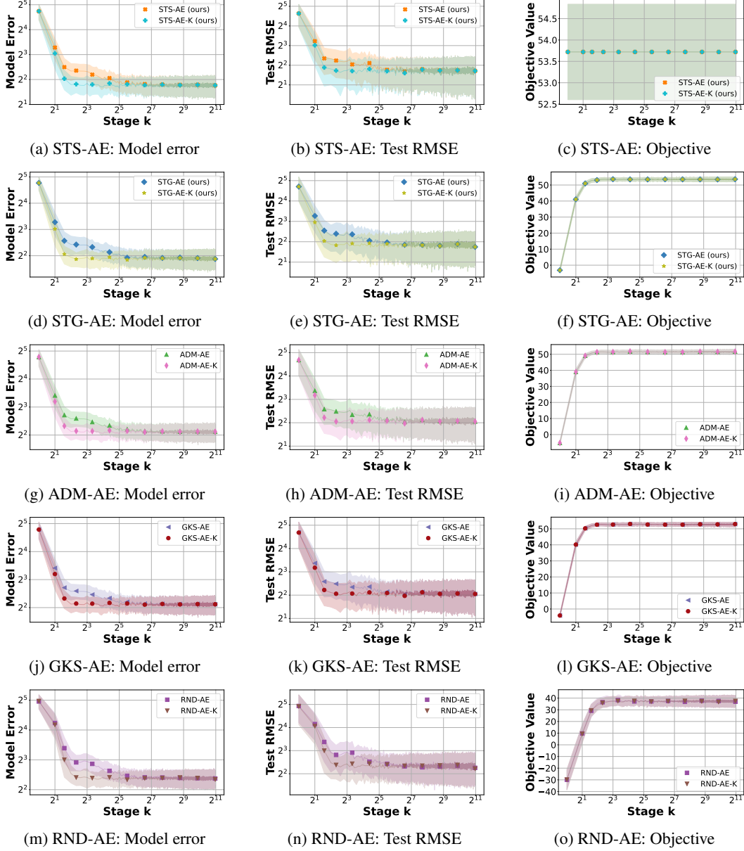
Figure 13: Unknown vs. known \beta_* comparisons across the five AE methods in synthetic sub-scenario II. Rows (top to bottom) correspond to the five AE methods: STS-AE, STG-AE, ADM-AE, GKS-AE, RND-AE. Columns (left to right) correspond to: model error (Eq. (147)) between the estimation \hat{\beta}_{k|k} and the true model \beta_k , lower is better; test RMSE (Eq. (145)) between predicted labels \mathbf{y}_k^{\text{pred}} and test labels \mathbf{y}_k^{\text{test}} , lower is better; objective value (Eq. (150)), higher is better (maximization problem). Shaded regions represent \pm 1 standard deviation from the mean.
