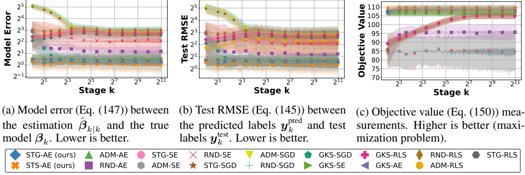
Figure 10: Performance w.r.t. model error, test RMSE, and objective value for synthetic sub-scenario I as a function of the stage k . Shaded regions represent \pm 1 standard deviation from the mean. We observe that our methods STG-AE and STS-AE achieve lower model error and test RMSE, as well as higher objective value compared to other methods.
