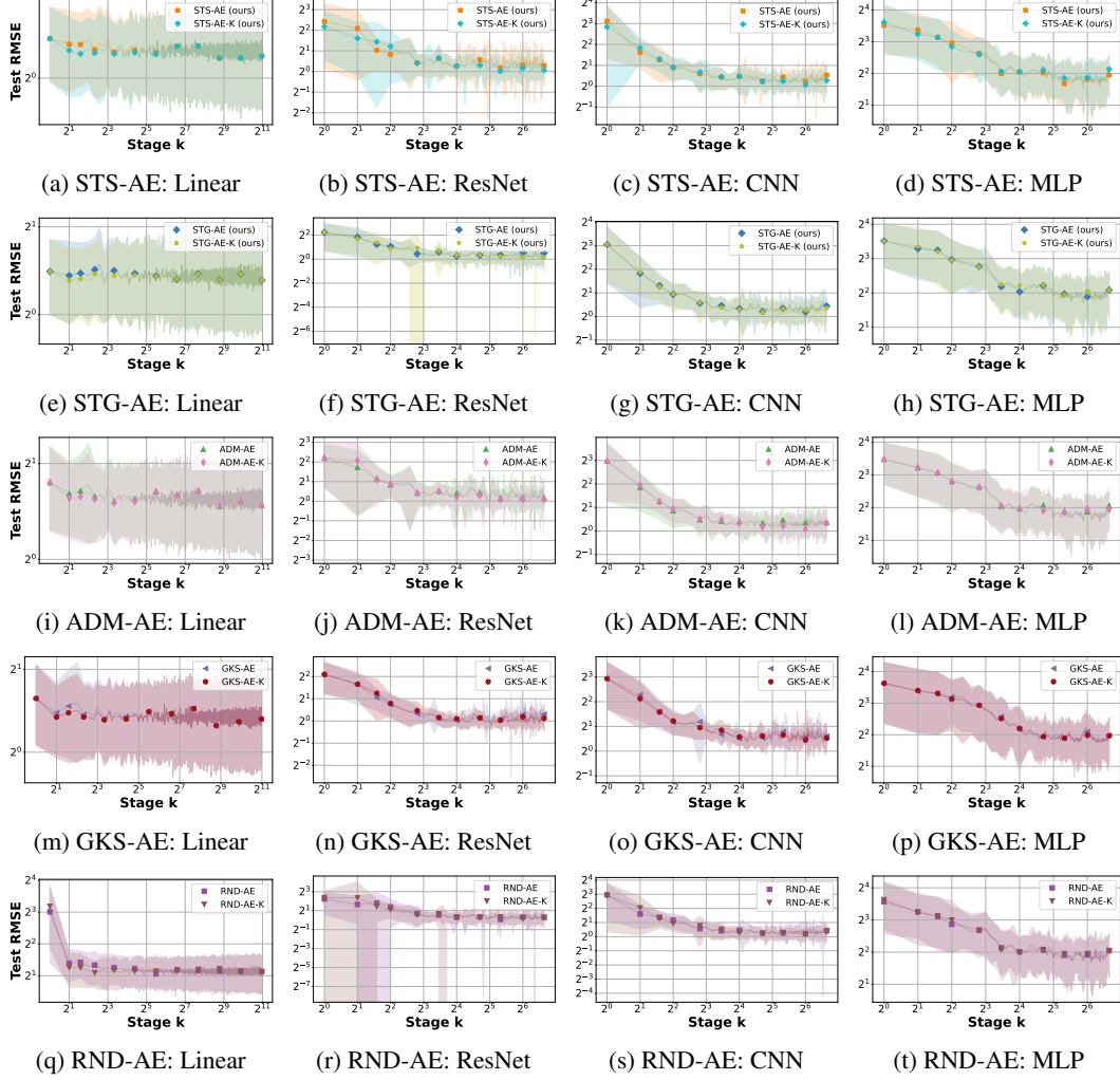
Figure 7: Unknown vs. known \beta_* test RMSE comparisons across the five AE methods on the synthetic dataset; lower is better. Rows (top to bottom) correspond to the five AE methods: STS-AE, STG-AE, ADM-AE, GKS-AE, RND-AE. Columns (left to right) correspond to the four model architectures: Linear, ResNet, CNN, MLP. Shaded regions represent \pm 1 standard deviation from the mean.
