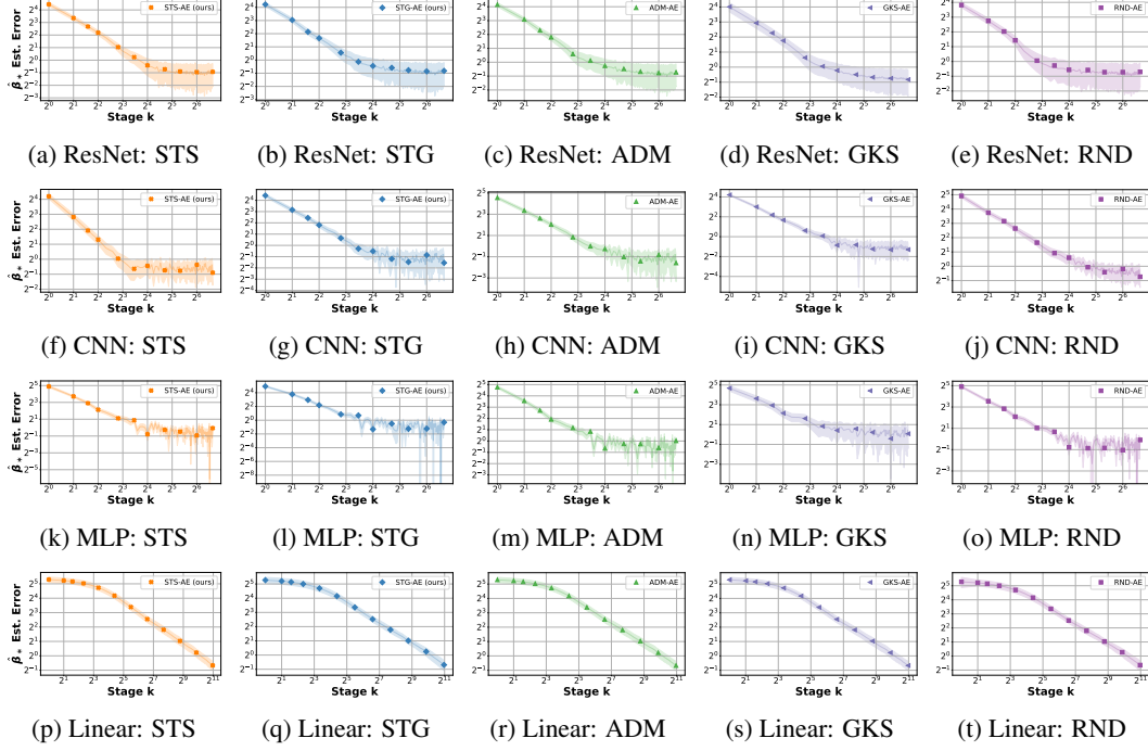
Figure 6: Estimation error between the estimation \hat{\beta}_* and the true mean fixed-point \beta_* for the AE methods on the synthetic dataset, across four model architectures (rows, top to bottom: ResNet, CNN, MLP, Linear) and five AE methods (columns, left to right: STS-AE, STG-AE, ADM-AE, GKS-AE, RND-AE). Shaded regions represent \pm 1 standard deviation from the mean.
