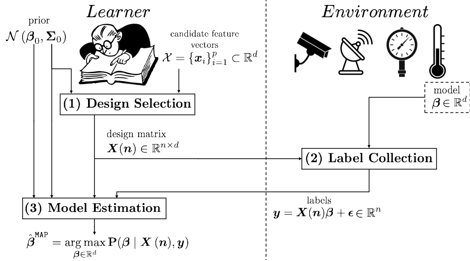
Figure 3: The classic experimental design setting. A learner having access to a prior distribution \mathcal{N}(\beta_0, \Sigma_0) wishes to determine which experiments to conduct to estimate (hidden) model \beta . The entire process comprises three steps. In the design selection step, the learner selects n experiments to conduct, resulting in design matrix \mathbf{X}(\mathbf{n}) \in \mathbb{R}^{n \times d} . In the label collection step, corresponding experiments are conducted and labels \mathbf{y} \in \mathbb{R}^n are revealed. In the model estimation step, the model is estimated via maximum a posteriori estimation. Only the covariance of the model prior is used in design selection, while the full prior is used in model estimation. In D-Optimal design, the design selection is determined by selecting samples that minimize the entropy of the posterior.
