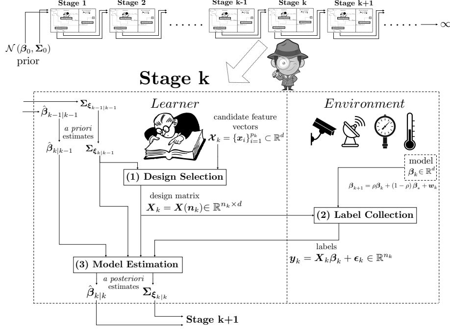
Figure 4: Our proposed Markovian experimental design setting. The experimental design scenario is repeated over multiple stages, during which the underlying model is subject to drift, as determined by Eq. (59). Compared to Fig. 3, the posterior from the previous stage (whose parameters are indicated by (\cdot)_{k-1|k-1} ) is used to compute the prior at the next stage (indicated by (\cdot)_{k|k-1} ), via Eq. (61). Note that these are not identical, as the model has drifted from stage k-1 to stage k . Moreover, model estimation is full-Bayesian, rather than a MAP estimate of \beta_k : through Eq. (62), the learner estimates the full posterior (i.e., both mean and variance, indicated by (\cdot)_{k|k} ). This happens through a Kalman filter estimation process. As a result, the posterior estimated is in fact the posterior after seeing the entirety of observations \{(\mathbf{X}_{k'}, \mathbf{y}_{k'})\}_{k'=1}^k . Our analysis answers the question of how to optimally perform the design selection step in this setting (i.e., how to choose \mathbf{n}_k ), either per-stage k or asymptotically, i.e., in steady-state.
