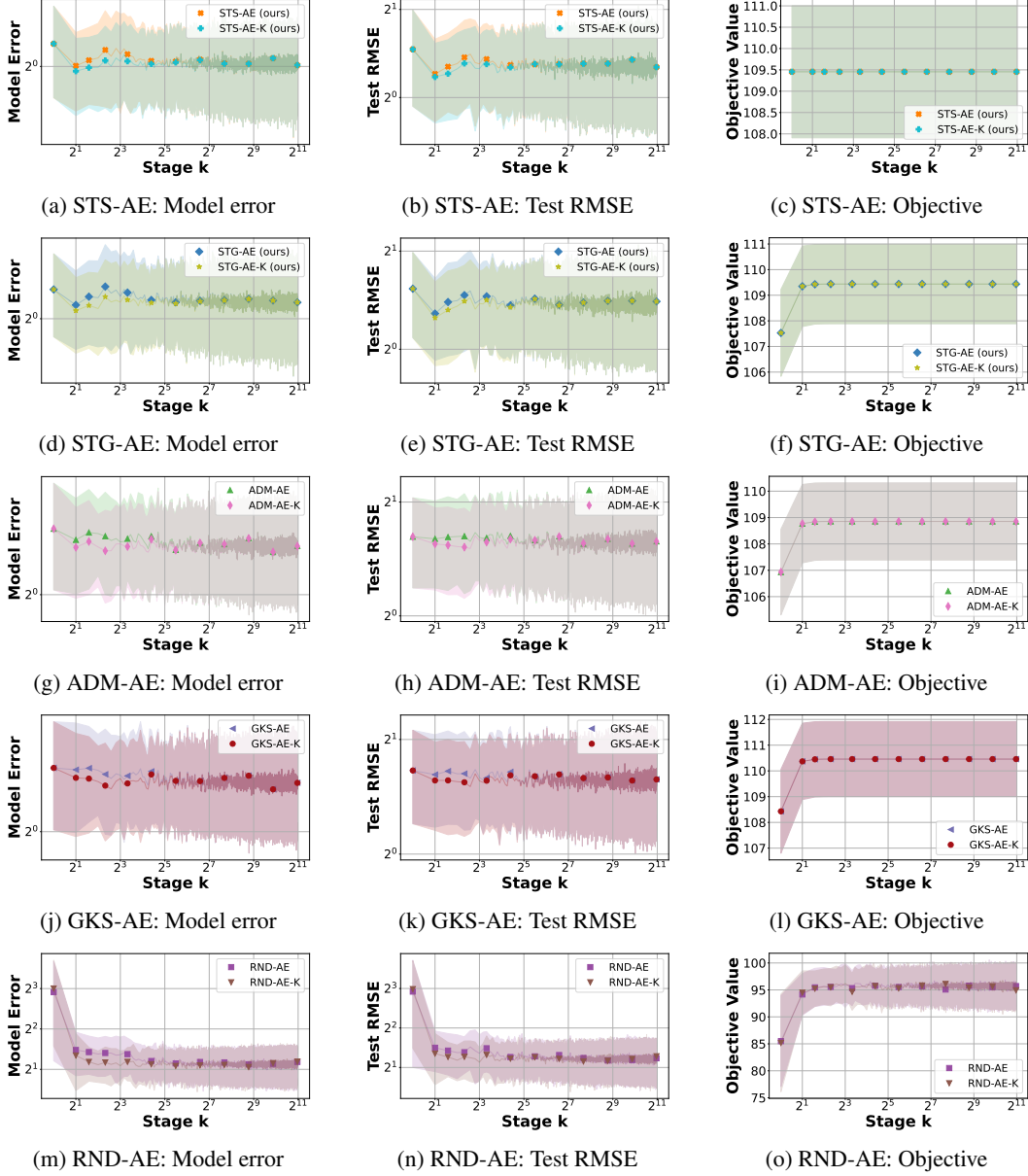
Figure 12: Unknown vs. known \beta_* comparisons across the five AE methods in synthetic sub-scenario I. Rows (top to bottom) correspond to the five AE methods: STS-AE, STG-AE, ADM-AE, GKS-AE, RND-AE. Columns (left to right) correspond to: model error (Eq. (147)) between the estimation \hat{\beta}_{k|k} and the true model \beta_k , lower is better; test RMSE (Eq. (145)) between predicted labels y_k^{\text{pred}} and test labels y_k^{\text{test}} , lower is better; objective value (Eq. (150)), higher is better (maximization problem). Shaded regions represent \pm 1 standard deviation from the mean.
