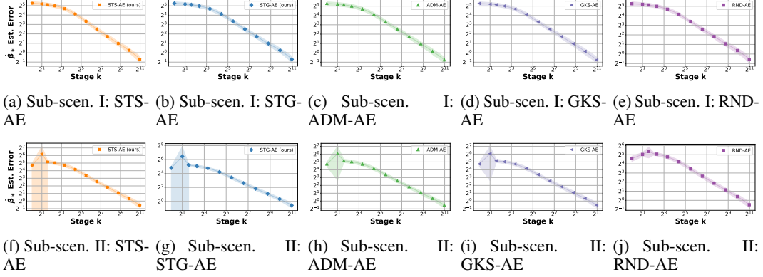
Figure 11: Estimation error between the estimation \hat{\beta}_* and the true mean fixed-point \beta_* for the AE methods on the synthetic dataset. Rows (top to bottom) correspond to the two synthetic sub-scenarios: Sub-scenario I and Sub-scenario II. Columns (left to right) correspond to the five AE methods: STS-AE, STG-AE, ADM-AE, GKS-AE, RND-AE. Shaded regions represent \pm 1 standard deviation from the mean.
