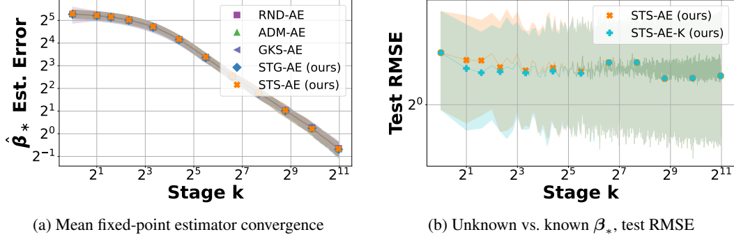
Figure 1: Representative results for the linear measurement model on the synthetic dataset. (a) Estimation error between \hat{\beta}_* and the true mean fixed-point \beta_* ; lower is better. (b) Test RMSE for the STS-AE method when \beta_* is unknown (estimated online) vs. known; lower is better. Shaded regions represent \pm 1 standard deviation from the mean.
