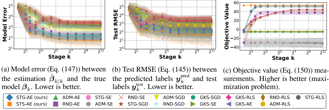
Figure 14: Performance w.r.t. model error, test RMSE, and objective value for synthetic sub-scenario II as a function of the stage k . Shaded regions represent \pm 1 standard deviation from the mean.
