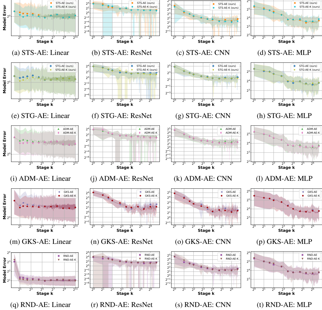
Figure 8: Unknown vs. known \beta_* model error comparisons across the five AE methods on the synthetic dataset; lower is better. Rows (top to bottom) correspond to the five AE methods: STS-AE, STG-AE, ADM-AE, GKS-AE, RND-AE. Columns (left to right) correspond to the four model architectures: Linear, ResNet, CNN, MLP. Shaded regions represent \pm 1 standard deviation from the mean.
