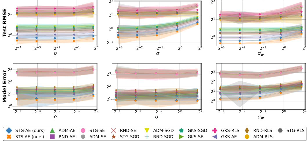
Figure 2: Test RMSE (Eq. (145), top row) and model error (Eq. (148), bottom row) comparisons with respect to different values of \rho , \sigma , and \sigma_w on the synthetic dataset for the ResNet model; other parameters as in Table 4. Lower is better. Shaded regions represent \pm 1 standard deviation from the mean.
