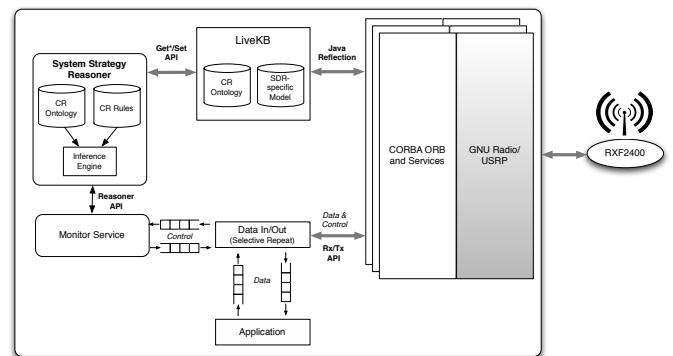
Figure 2. Implementation Architecture
