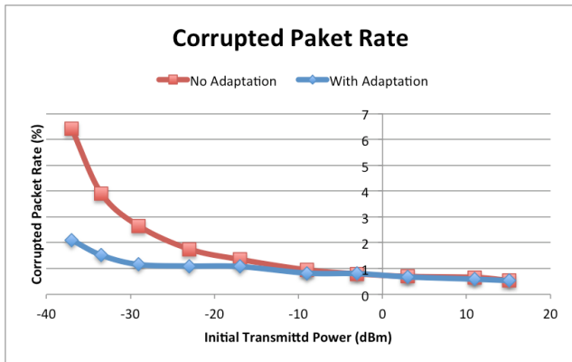
Figure 6 Performance Evaluation (3): Corrupted Packet Rate
