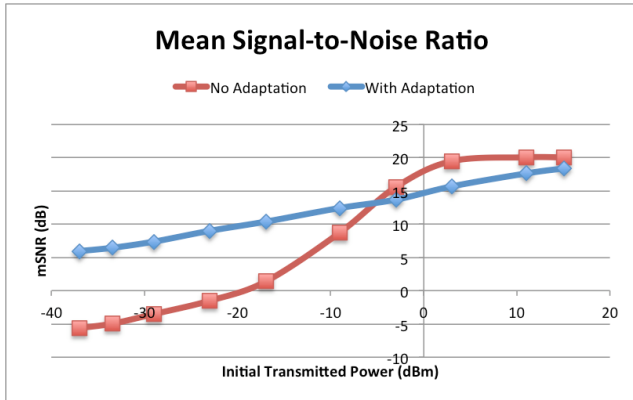
Figure 4 Performance Evaluation (1): Mean SNR
