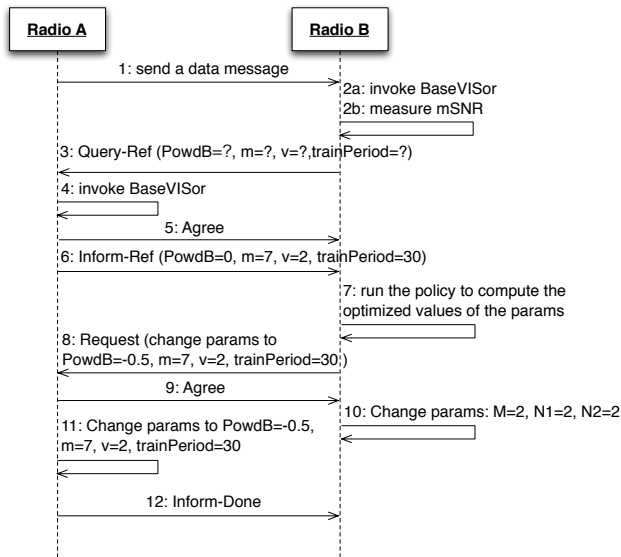
Figure 3. Sequence Diagram of Link Optimization
