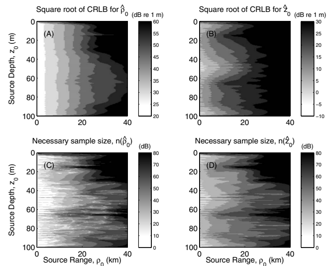
FIG. 13. The same as Fig. 9, but here the mean \mu of the measurement is assumed parameter independent so that its derivatives in Eqs. (12) and (13) are set to zero. The CRLB and the sample sizes necessary to attain it are overestimated when compared with Fig. 9. This scenario is equivalent to incorrectly assuming the received measurement is purely random with zero mean, embedded in additive white noise.
