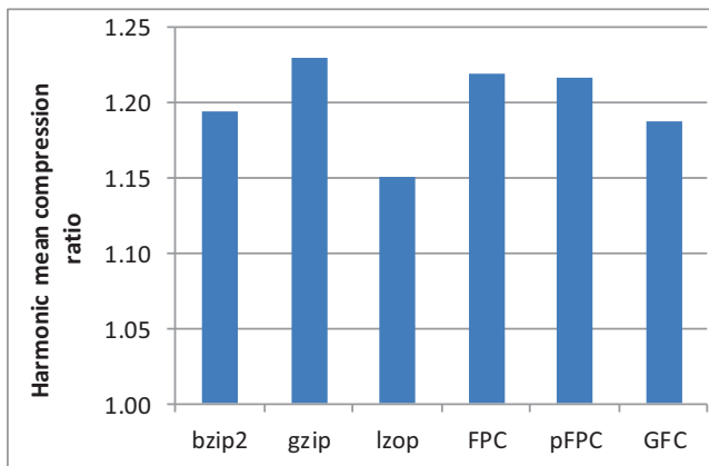
Figure 4. Harmonic-mean compression ratio of six algorithms sorted from slowest (leftmost) to fastest (rightmost)
