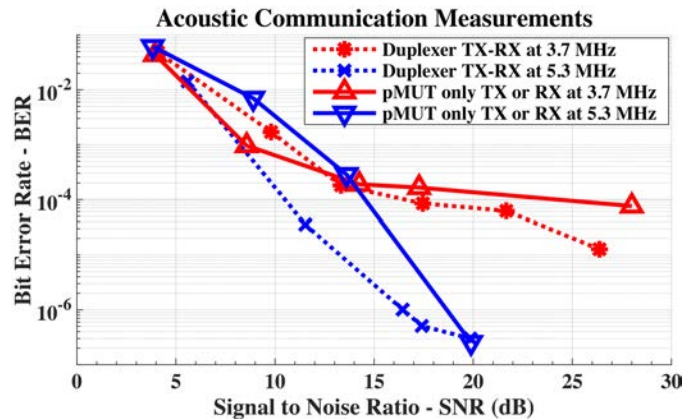
Fig. 6. Acoustic communication measurements of the Bit-Error-Rate ( BER ) vs. the Signal-to-Noise Ratio ( SNR ). The solid lines are the measurements with pMUTs arrays only while the dashed lines are the measurements with the duplexers added to the communication system. Red and blue lines are the communication results through the f_1 = 3.7MHz and f_2 = 5.3MHz bandwidths of the duplexer respectively. (TX = Transmit, RX = Receive)
