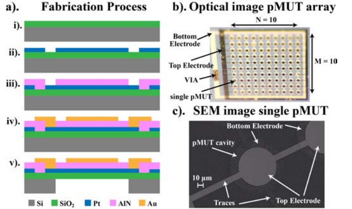
Fig. 3. a). pMUTs array fabrication process steps. (i) SiO_2 thermal growth. (ii) Bottom electrode deposition ( Pt ) and patterning. (iii) AlN deposition. (iv) Top electrode deposition ( Au ) and patterning. (v) Backside etching to define the pMUTs cavity and membrane area. b). Optical image of a fabricated pMUTs array. The array is made by N = 10 columns and M = 10 rows, thus a 100 pMUTs in total. Top and bottom traces together with the VIAs can be distinguished in the figure. c). Scanning Electron Microscope (SEM) image of a single pMUT. Top and bottom electrodes and traces together with the pMUT cavity can be distinguished in the figure.
