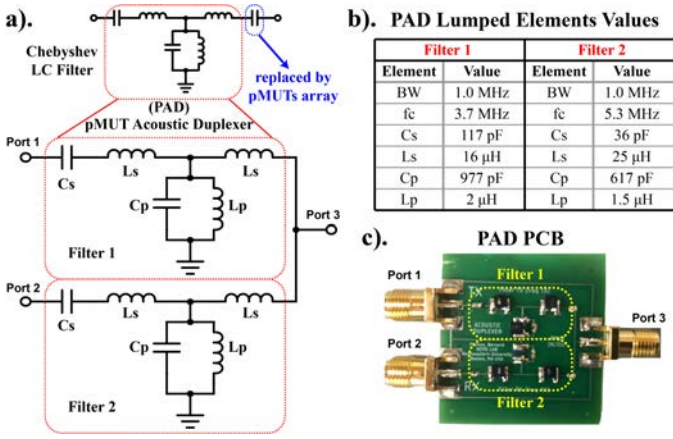
Fig. 1. a). At the top is shown a typical LC-tree configuration for a band-pass Chebyshev filter where the last series capacitance is replaced by the pMUT array capacitance. At the bottom is shown the configuration of the pMUT Acoustic Duplexer (PAD) used in this work. b). Table of the PAD lumped elements values for both modified band-pass Chebyshev filters. The filters are designed with center frequencies ( f_c ) f_1 = 3.7MHz and f_2 = 5.3MHz respectively, and bandwidths of 1MHz each. c). PCB of the PAD prototype used in this work. The two filters are highlighted with the yellow dashed line and the input (Port 1 and Port 2) and output (Port 3) ports are marked.
